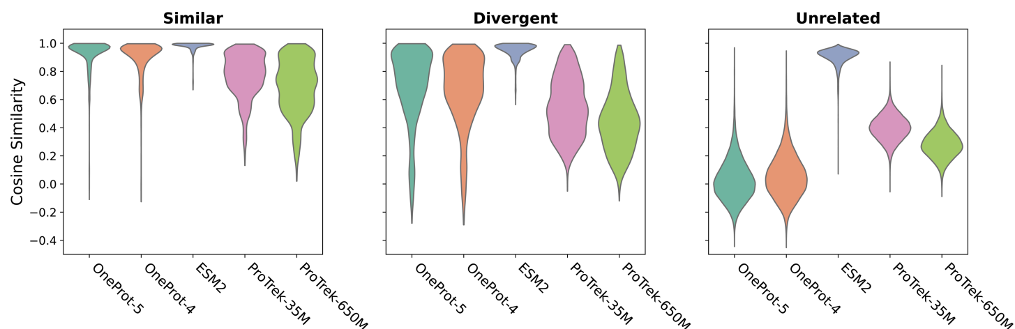
Fig 5. Cosine Similarity distributions for models ESM-2, ProTrek-35M and -650M, OneProt-4 and -5. The plot shows the similarity of a given protein to three groups: the 50 most evolutionarily similar proteins, the 50 most evolutionarily divergent sequences, and 1000 unrelated sequences. While all models partially capture evolutionary relationships, OneProt distinctly separates the three classes, demonstrating its ability to generate meaningful sequence representations.
